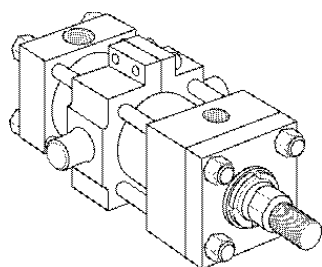
Style DD Intermediate Fixed Trunnion (NFA Style MT4)
