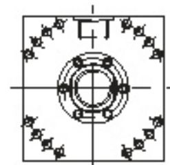
304.8mm (12") Bore Design 16 Tie Rod Construction
